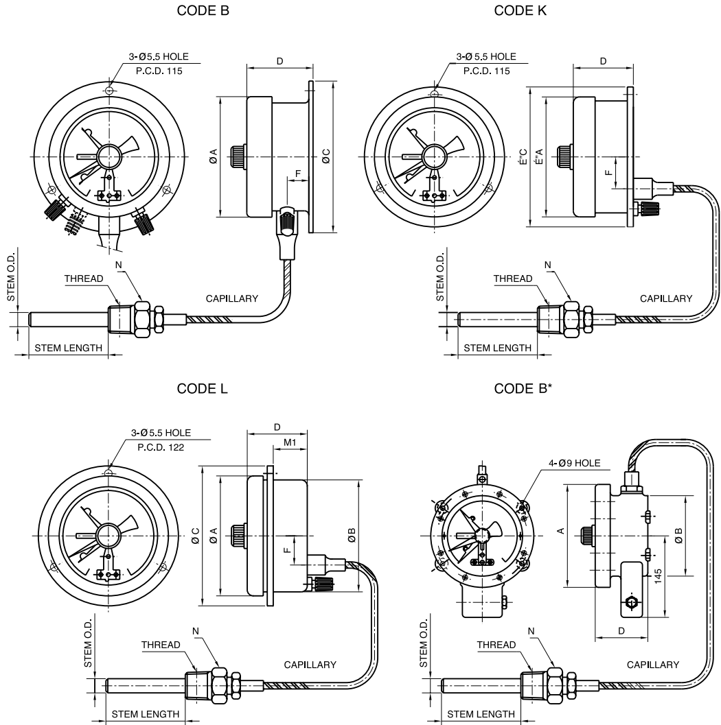
Dimensions (mm)
