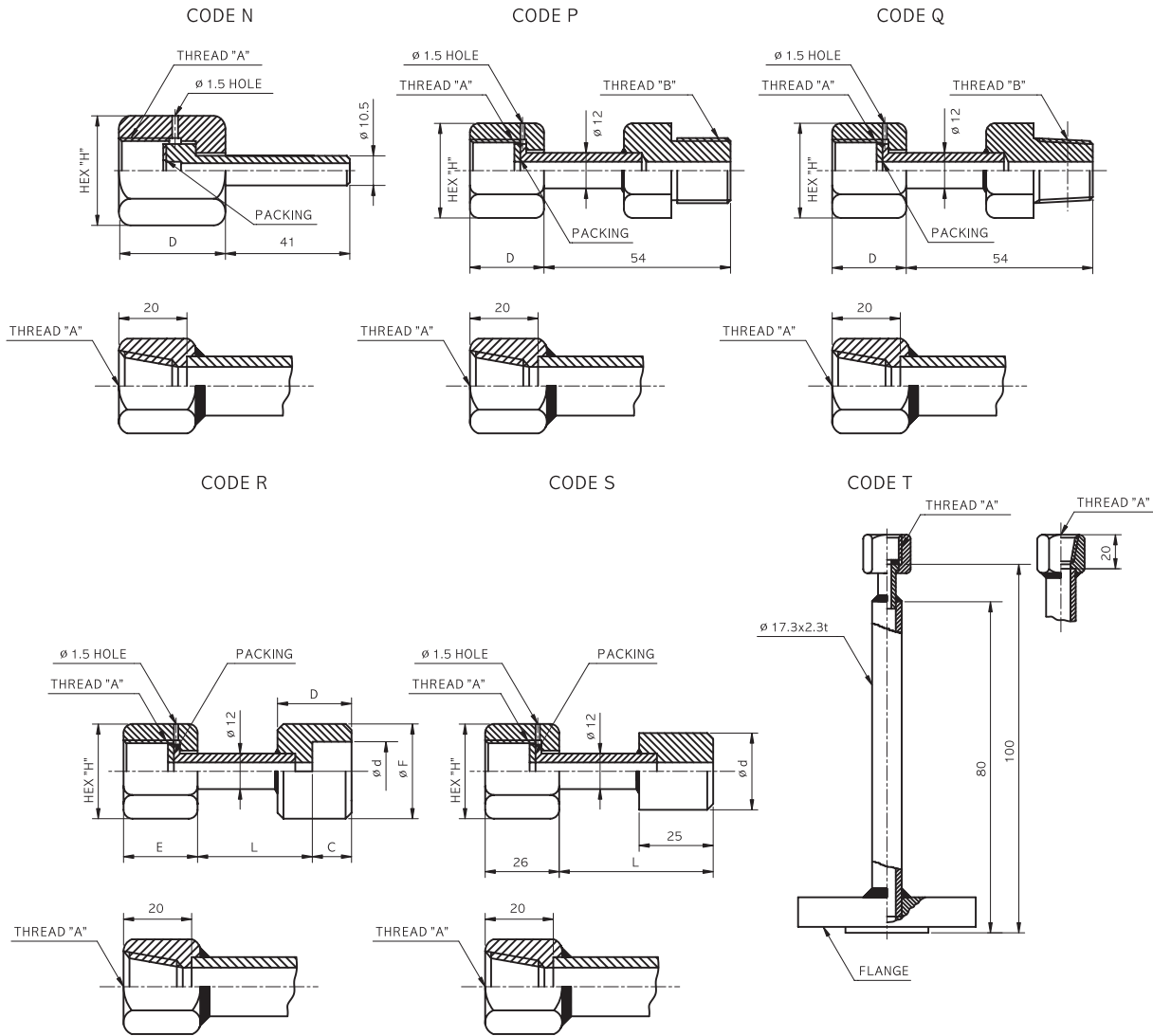
Dimensions (mm)
